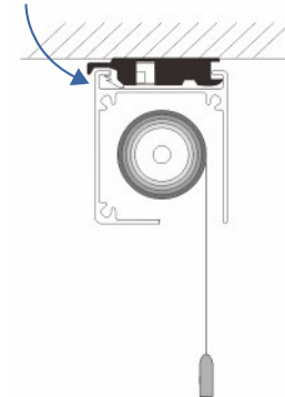
SIDE VIEW Top Structure Situation A
