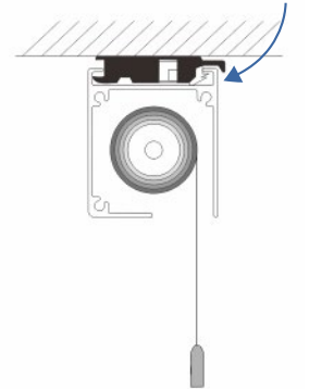
SIDE VIEW Top Structure Situation B
